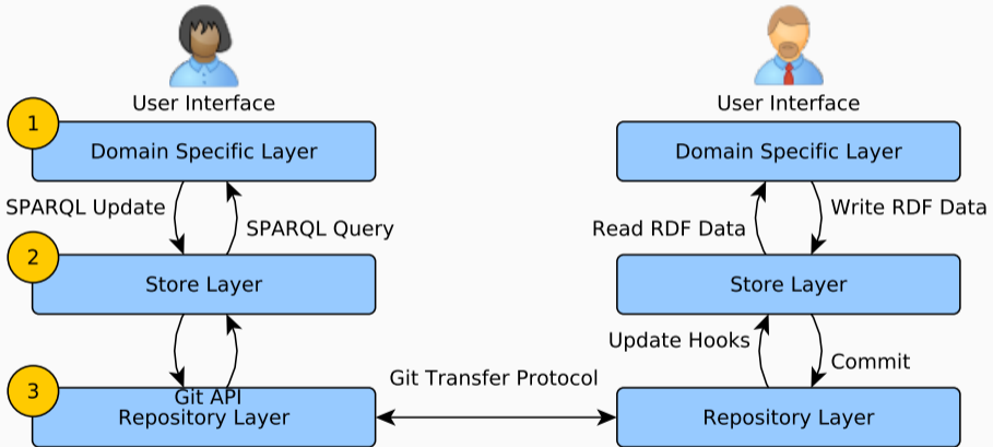
Figure 2: The functions and flow of information
